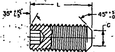
(B) SELF-LOCKING ELEMENT (SEE NOTE 6)
